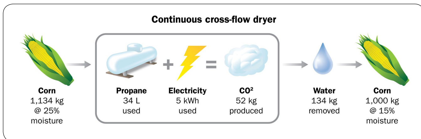
Figure 2. Approximate fuel used and carbon dioxide emissions produced to dry one tonne of corn from 25% to 15% moisture using a continuous cross-flow dryer.
