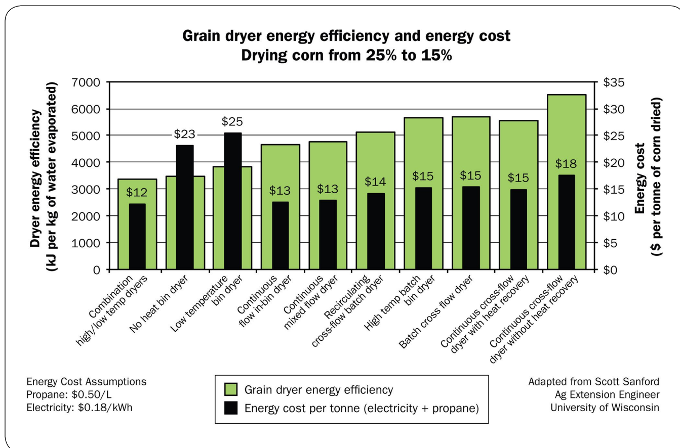
Figure 3. Approximate efficiencies and operating costs for different grain dryers. Numbers are based on drying one tonne of corn from 25% to 15% moisture. Costs include fuel (propane) and electricity. Source: Scott Sanford, M. Eng., University of Wisconsin-Madison, USA.
