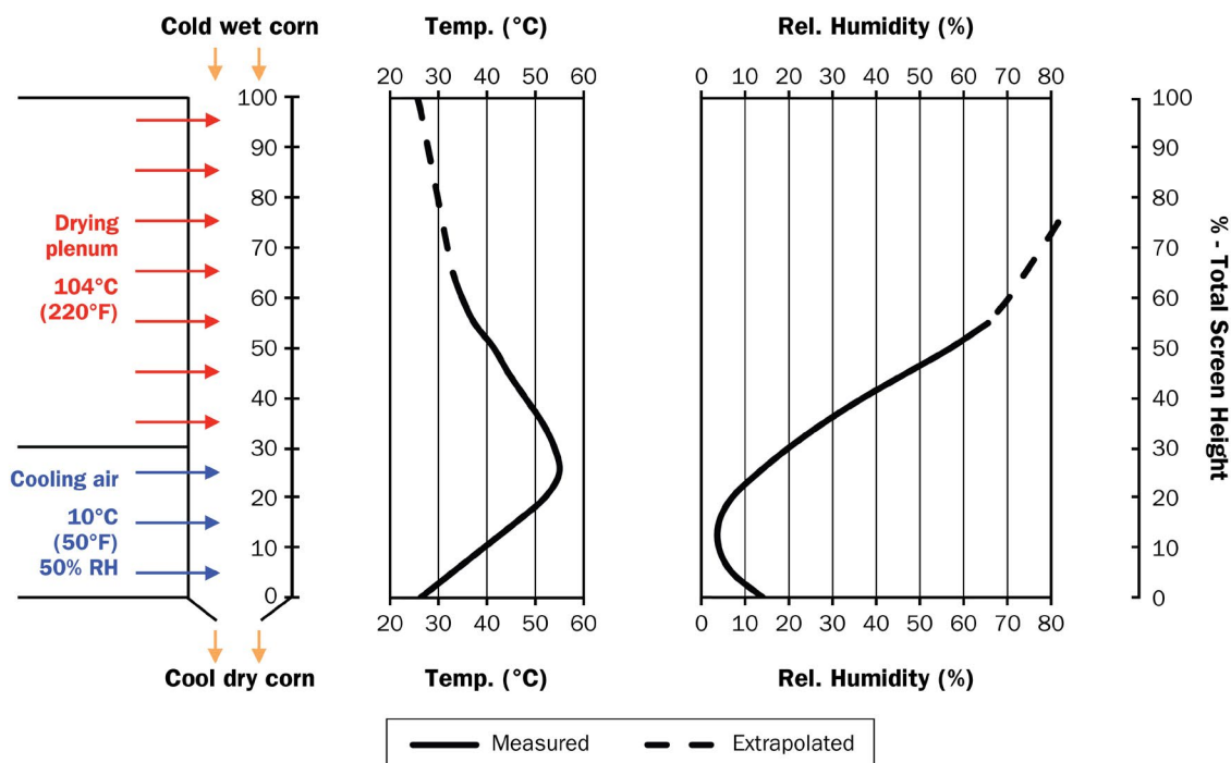
Figure 4. Approximate discharge air temperature and relative humidity profiles from a continuous cross-flow dryer with ambient air cooling. Warm, dry exhaust air can be recirculated to reduce energy use.
