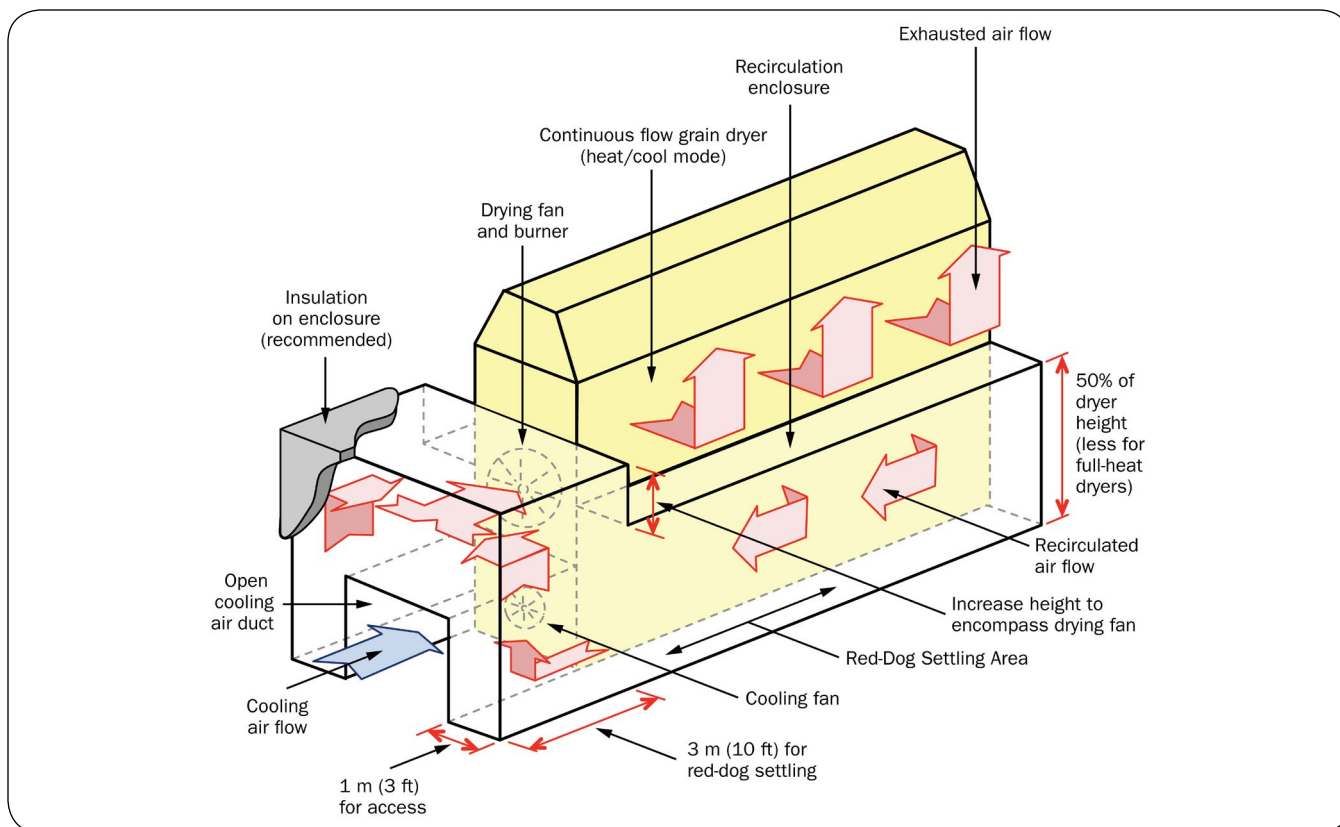
Figure 5. Example of a heat recirculation enclosure for a continuous flow dryer.
