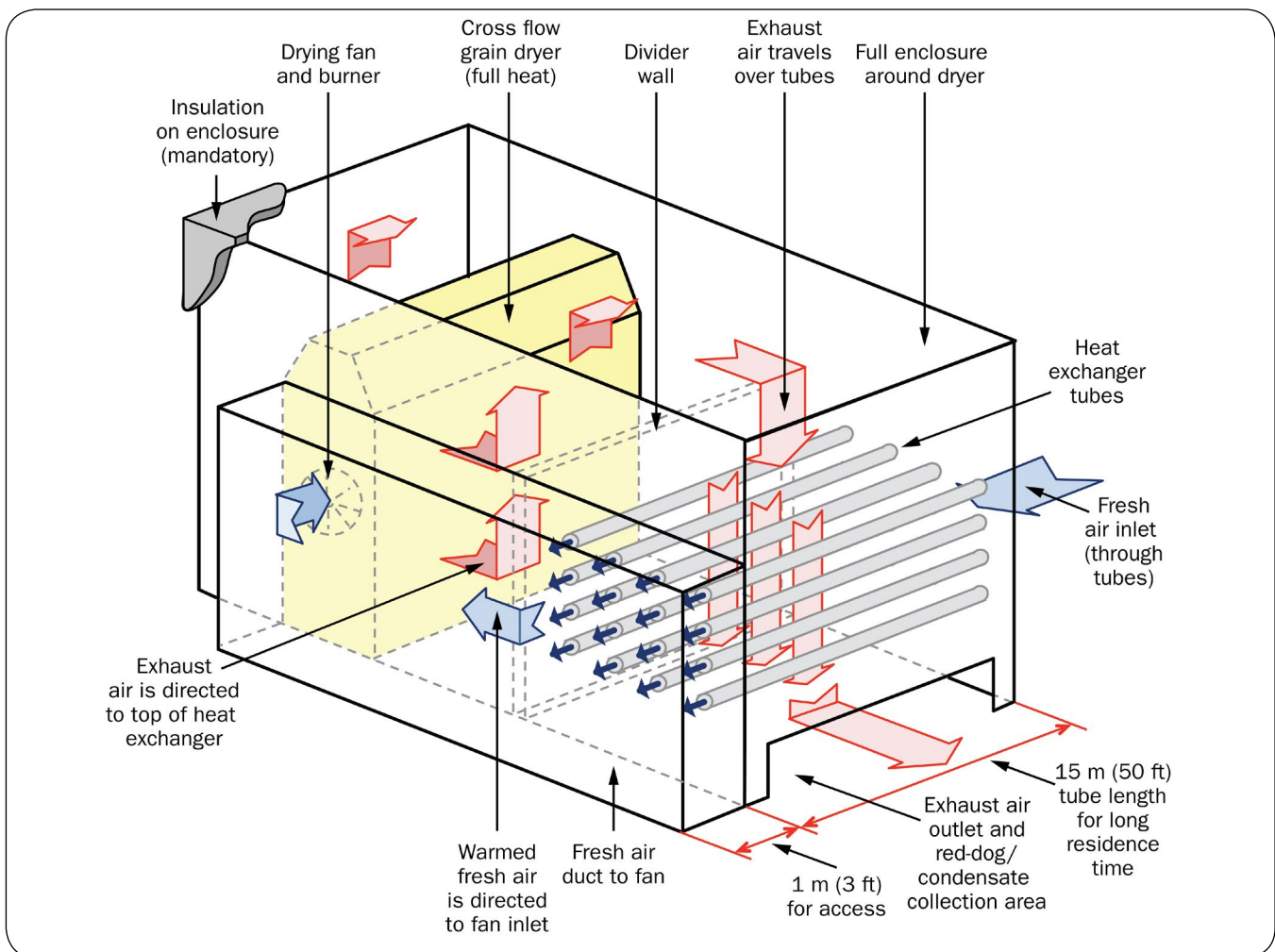
Figure 9. Example of a heat exchanger system for a continuous flow dryer.
