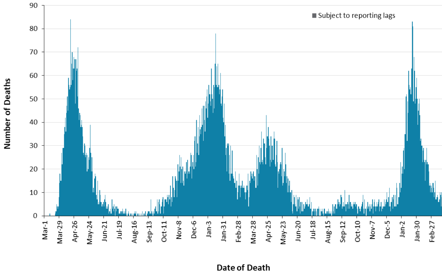
Figure 3. Confirmed deaths among COVID-19 cases by date of death: Ontario, March 1, 2020 to March 25, 2022
