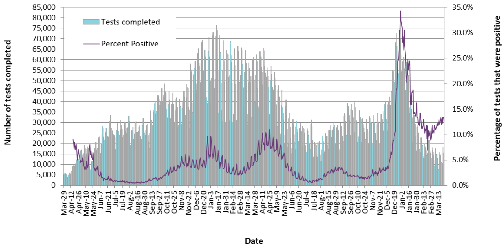
Figure 2. Number of COVID-19 tests completed and percent positivity: Ontario, March 29, 2020 to March 24, 2022
