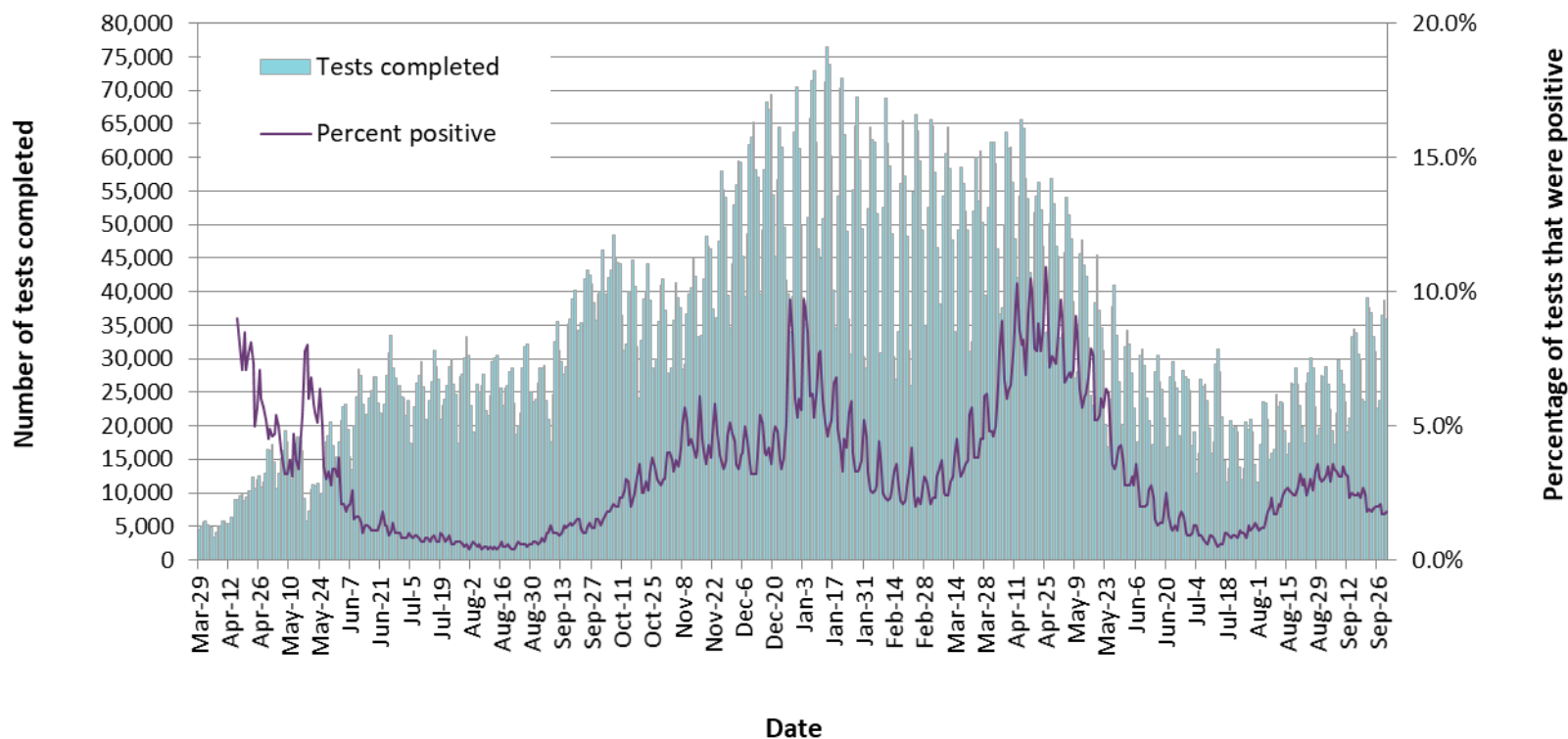
Figure 3. Number of COVID-19 tests completed and percent positivity: Ontario, March 29, 2020 to September 30, 2021
