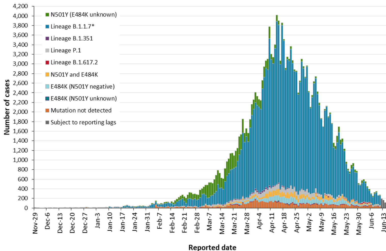
Figure 6. Confirmed COVID-19 cases with a mutation or VOC detected by public health unit reported date: Ontario, November 29, 2020 to June 16, 2021
