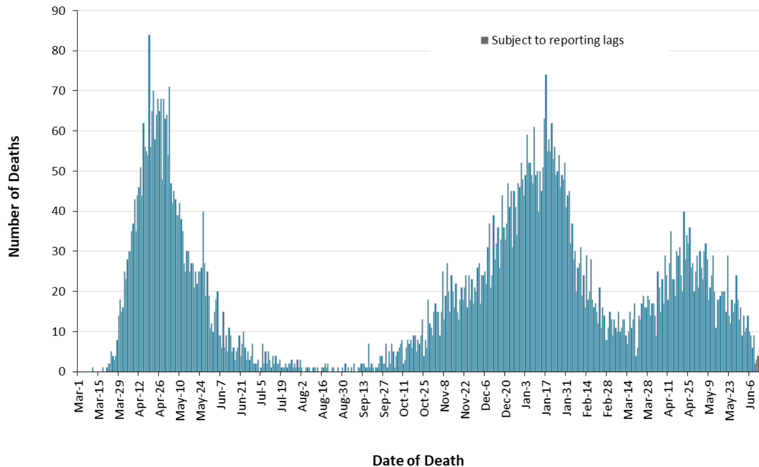
Figure 4. Confirmed deaths among COVID-19 cases by date of death: Ontario, March 1, 2020 to June 16, 2021
