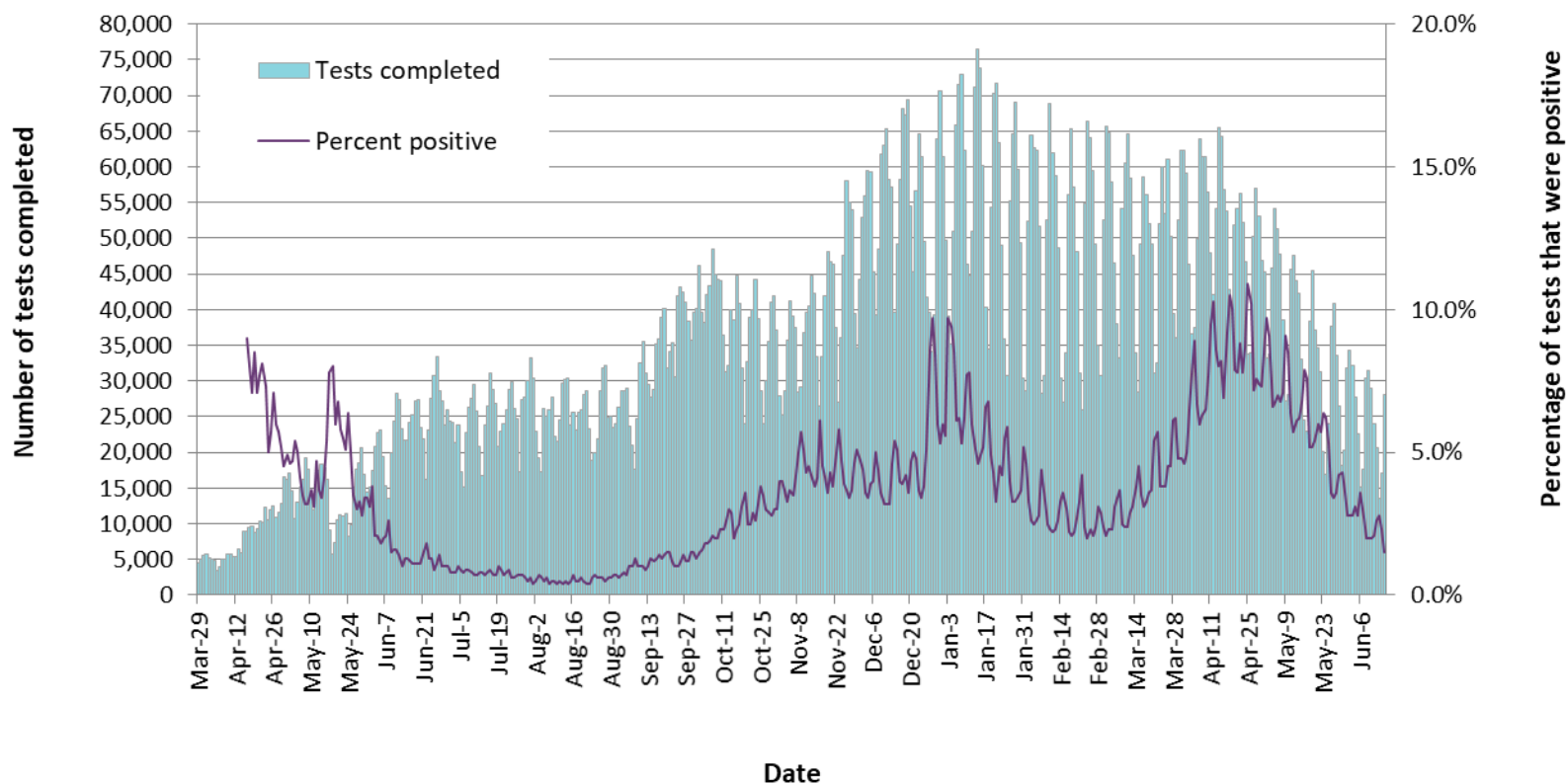
Figure 3. Number of COVID-19 tests completed and percent positivity: Ontario, March 29, 2020 to June 15, 2021
