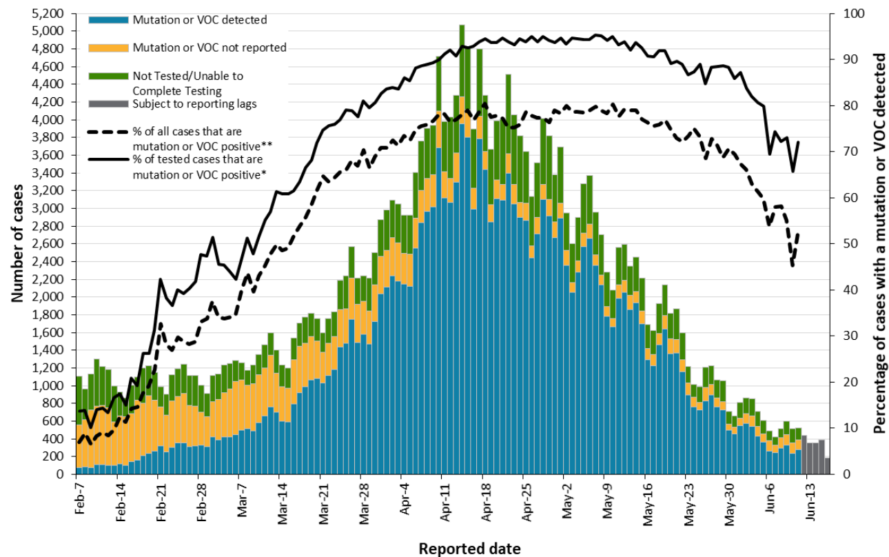
Figure 5. Number of confirmed COVID-19 cases and percent positive for mutations or VOCs: Ontario, February 7, 2021 to June 16, 2021
