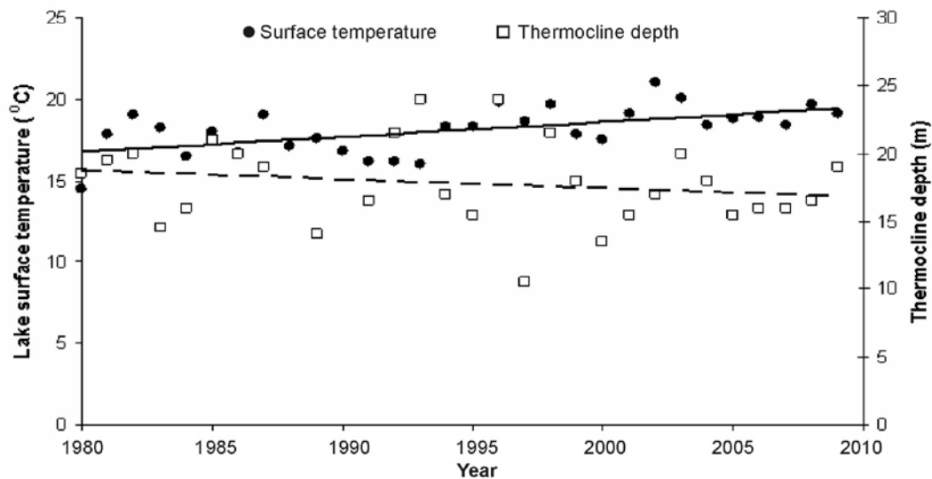
Figure 6. Surface water temperatures ( ^{\circ}\text{C} ) and thermocline depths (m) at station K42 in Kempenfelt Bay, Lake Simcoe from 1980 to 2009.
