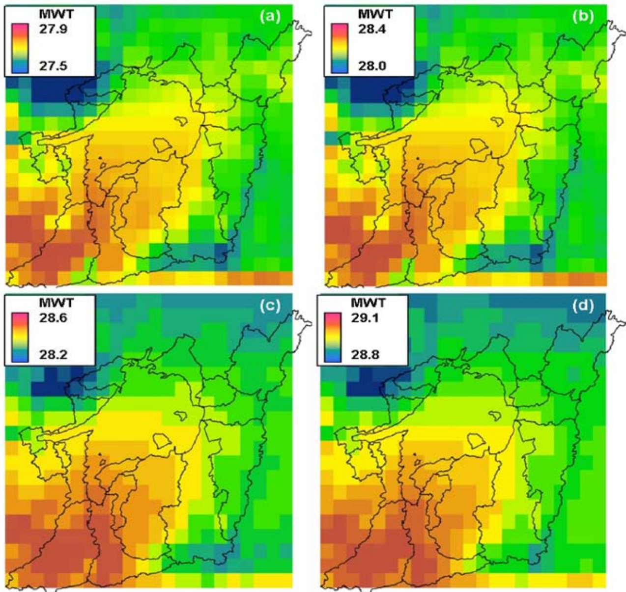
Figure 4. Maximum weekly stream temperatures (MWT) in the Lake Simcoe watershed under (a) current, (b) 2011-2040, (c) 2041-2070, and (d) 2071-2100 air temperature projections of the Canadian Global Climate Model 2 A2 scenario.
