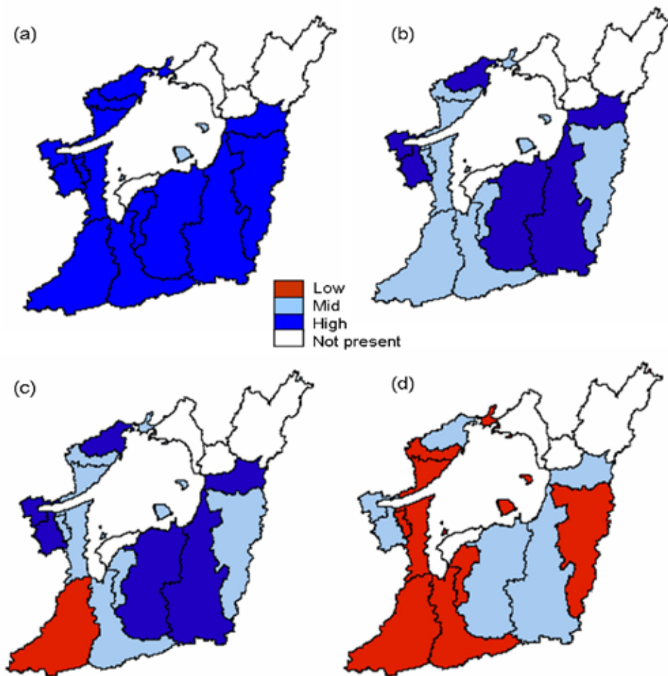
Figure 5. Likelihood that watersheds will retain coldwater fish species under the (a) current, (b) 2011-2040, (c) 2041-2070, and (d) 2071-2100 air temperature projections of the Canadian Global Climate Model 2 A2 scenario.
