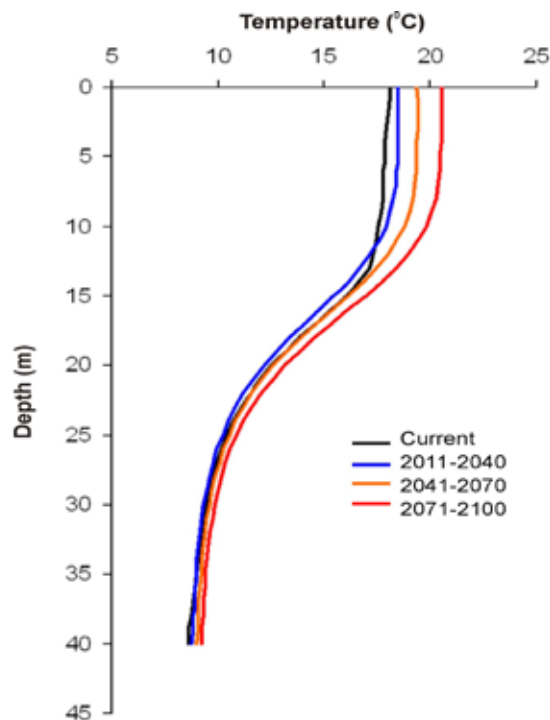
Figure 7. Estimated temperature profile for Kempenfelt Bay on September 15 under current and future climates based on the Canadian Global Climate Model 2 A2 and the temperature profile model outlined in Equation (1).
