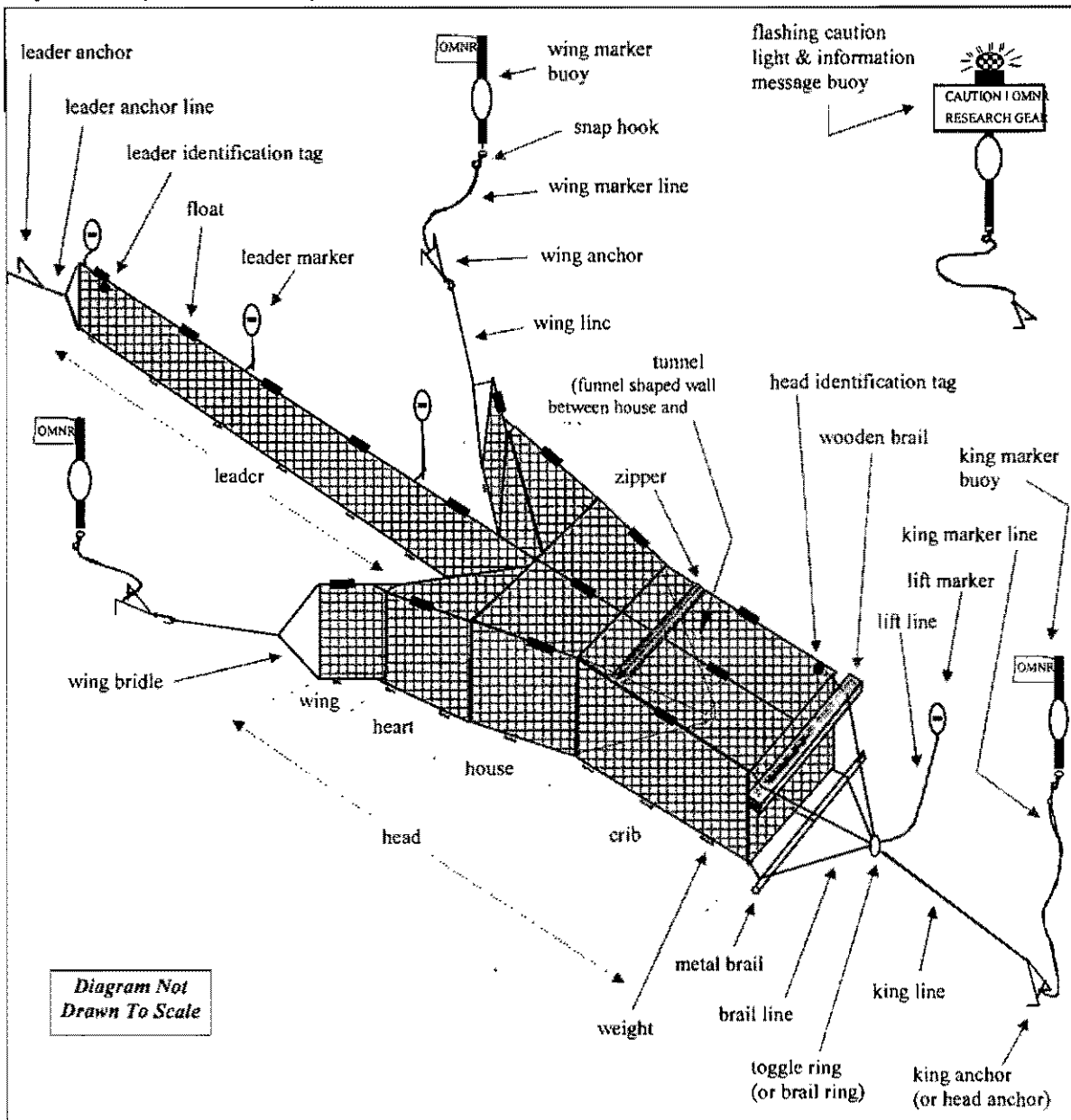
Figure 1: Spring-Haul Trap Net
